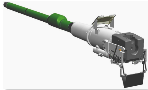
Fig. 3. Barrel mechanism of 120 mm K1A1 tank gun (Personal Fig).
