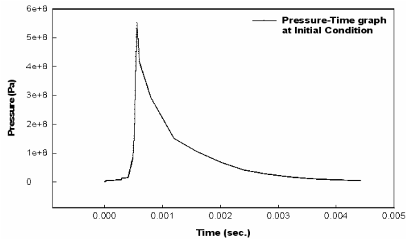
Fig. 5. Pressure-Time graph at inlet condition for 120 mm K1A1 tank gun.
