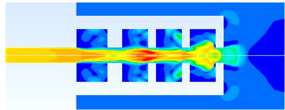
Fig. 8. Blast wave formation diagram inside the silencer.
