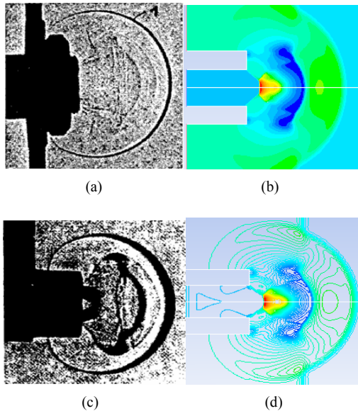
Fig. 1. (a) Reference shadow graph at t_{\text{exp}} \approx 2.5e-3\text{ms} ; (b) CFD Pressure graph; (c) Reference shadow graph at t_{\text{exp}} \approx 3.7e-3\text{ms} ; (d) CFD Pressure graph.
