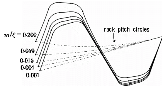
Fig. 13. Crown rack with respect to \alpha = 20^\circ and m/\xi = 0.000 \sim 0.200 .
