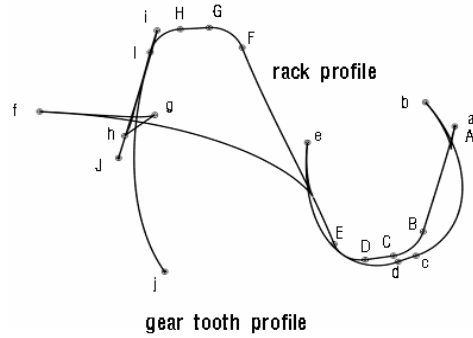
Fig. 18. Tooth profile with undercut ( m/\xi = 0.2, Z_g = 6, Z_{cr} = 9 ).
