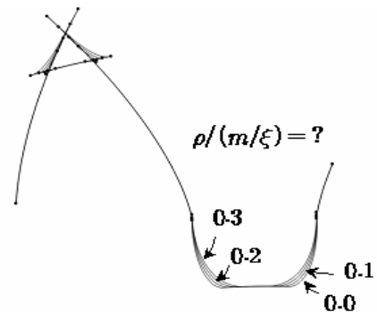
Fig. 16. Fillet curves along the radius of the round tip.
