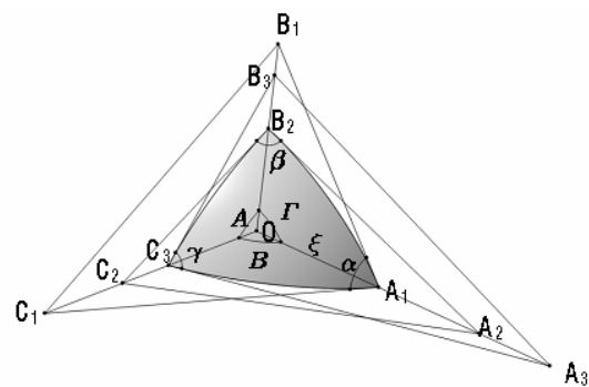
Fig. A.1. Spherical triangle and its relations.
