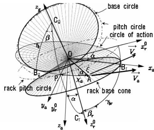
Fig. 7. Kinematic relationship between gear and basic rack.
