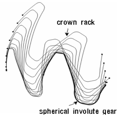
Fig. 15. Spherical involute gear generated by the crown rack ( m/\xi = 0.2, Z_g = 9 ).
