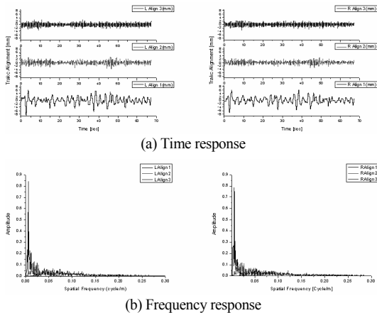
Fig. 10. Track alignment measurement results.
