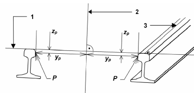
Fig. 4. Track alignment.
