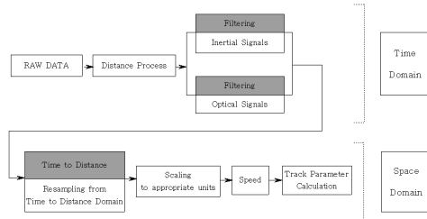
Fig. 6. Track measurement processing flow.
